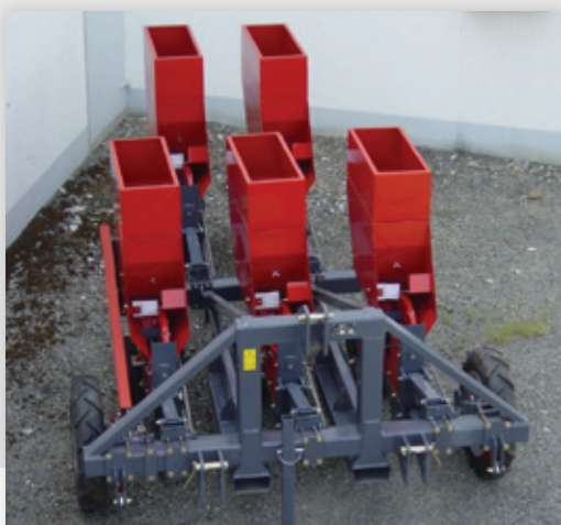
OPTION Special 25cm spacing equipment for onions
